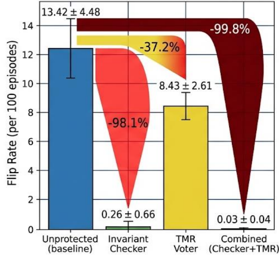
Figure 3. Ablation bar
